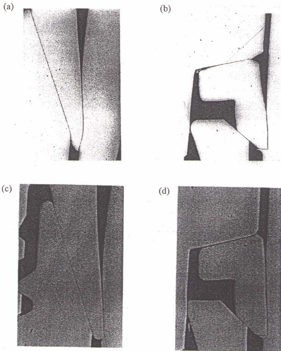
FIG. 9. (a) 'D' body, 'A' back ferrule, 'A' front ferrule and 'A' nut; (b) 'D' body, 'A' back ferrule, 'A' front ferrule and 'A' nut; (c) 'D' body, 'A' back ferrule, 'D' front ferrule and 'A' nut; (d) 'D' body, 'A' back ferrule, 'D' front ferrule and 'A' nut.
