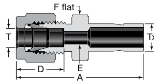
Reducer (Fractional to Metric)
