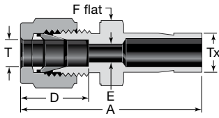
Reducer (Metric to Fractional)
