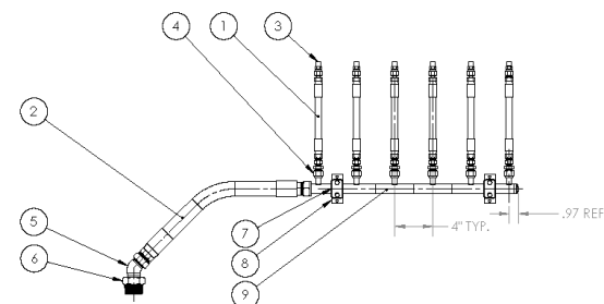
Concept Drawing
